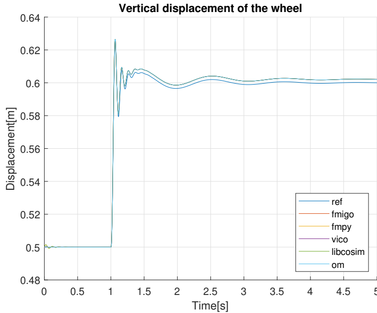
Figure 10: Wheel response when simulated at 1000hz.
