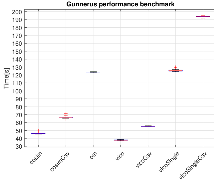
Figure 14: Performance of libcosim and Vico when considering the Gunnerus system. Simulation time=1000, step-size=0.05s, number of runs=10.
