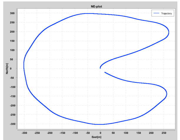
Figure 13: Demonstration of a vessel path following simulation running in Vico with 3D visualisation and plotting enabled.
