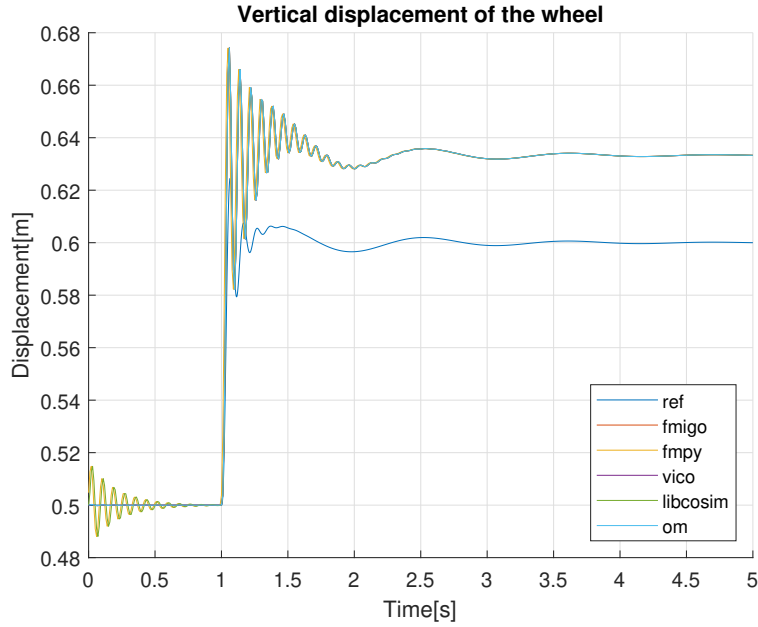
Figure 7: Wheel response when simulated at 100hz. The simulation starts from equilibrium state where z_w = 0 . The ground profile is defined as a step function excited by a jump of 0.1m in vertical direction at 1s .
