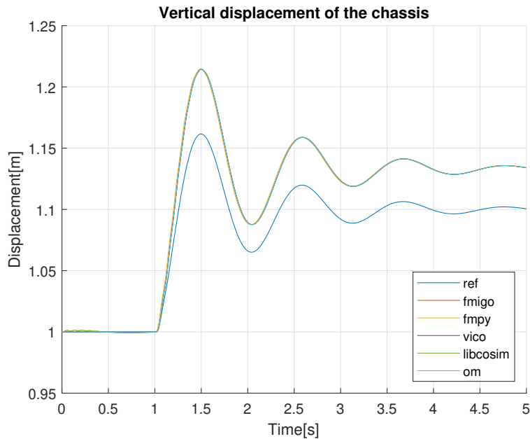
Figure 8: Chassis response when simulated at 100hz.
