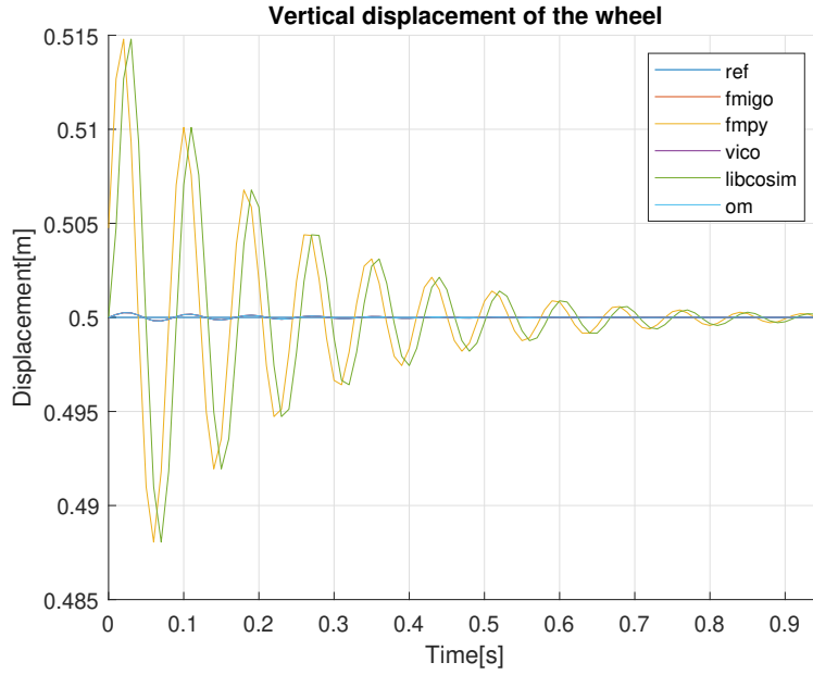
Figure 9: Detailed view of the the first second of simulation presented in Fig. 7.
