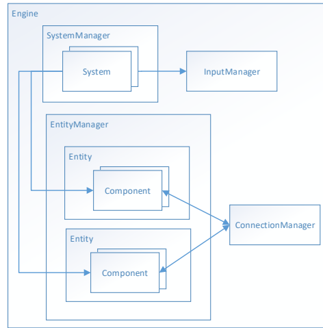
Figure 4: Composition of the various elements found in the Vico ECS implementation.
