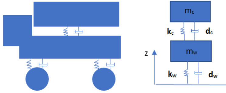
Figure 6: Illustration of the quarter-truck system.
