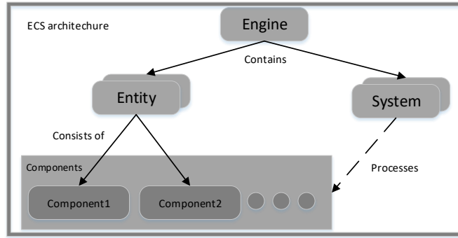
Figure 1: High level overview of the ECS architecture.
