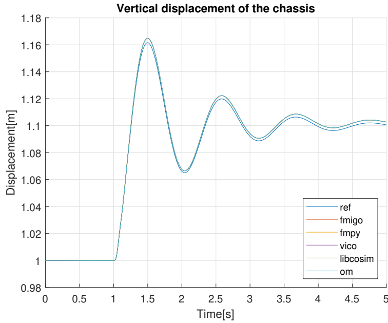
Figure 11: Chassis response when simulated at 1000hz.
