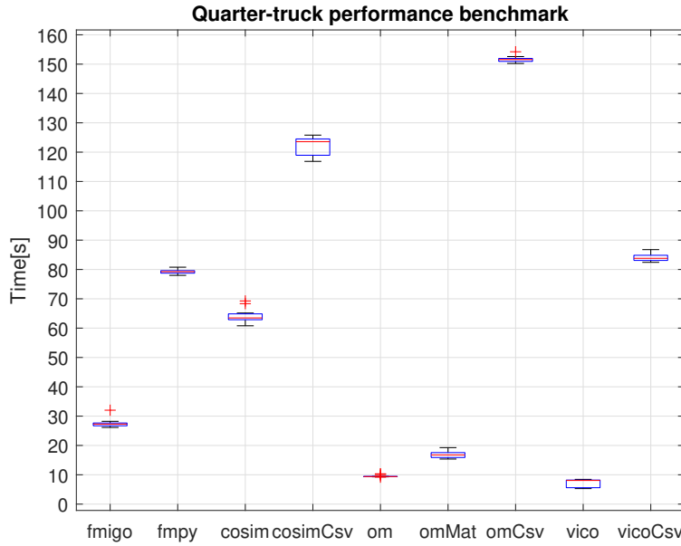
Figure 12: Performance of the various tools when considering the presented quarter-truck system. Simulation time=1000s, step-size=0.001s, number of runs=15.
