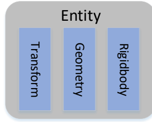
Figure 3: Anatomy of an entity. An entity is a collection of components. Components can be seamlessly added and removed, which effectively changes what the entity represents.
