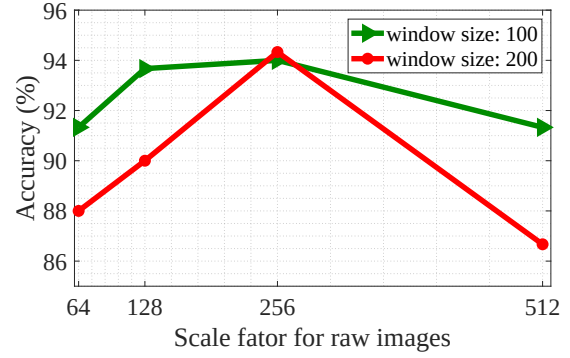
(a) Classification accuracy of different scale factors
